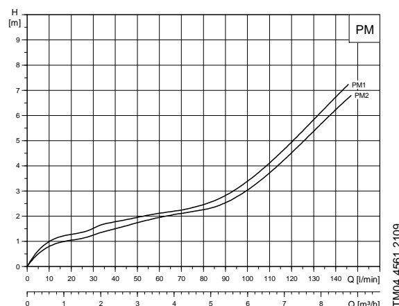
Fig. 12 Pressure loss curves for PM 1 and PM 2
