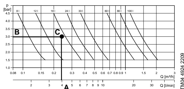
Fig. 9 Pressure tank selection curves
