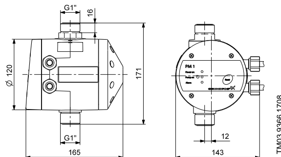
Fig. 10 Dimensional sketch of PM 1
